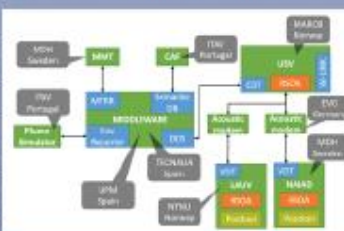
SWARMs SW integration
