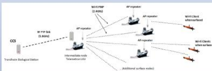
SWARMS communication system entities and nodes in Norway's final demo missions
