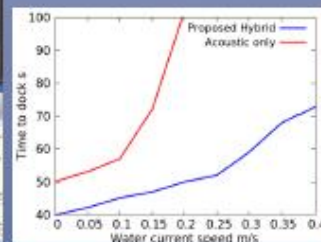
Time to dock vs. water current
