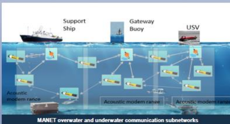
SWARMS communication system entities and nodes in Norway's final demo missions
